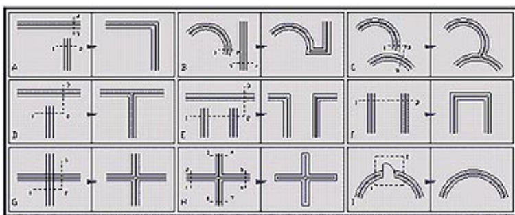
A=Blend Fillet, B=Blend Fillet, C=T.Junction, D=T.Junction, E=T.Junction, F=Cap, G=Chamfer, H=Cap, I=Chamfer
